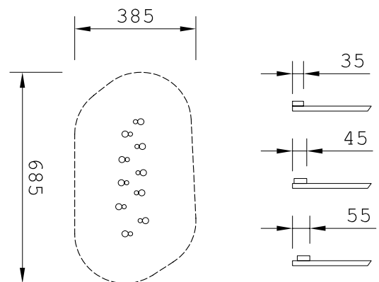
Plan View Not to scale
